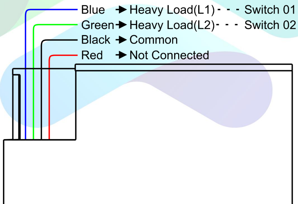
Smart Node Colour Wires to Switch Connection
