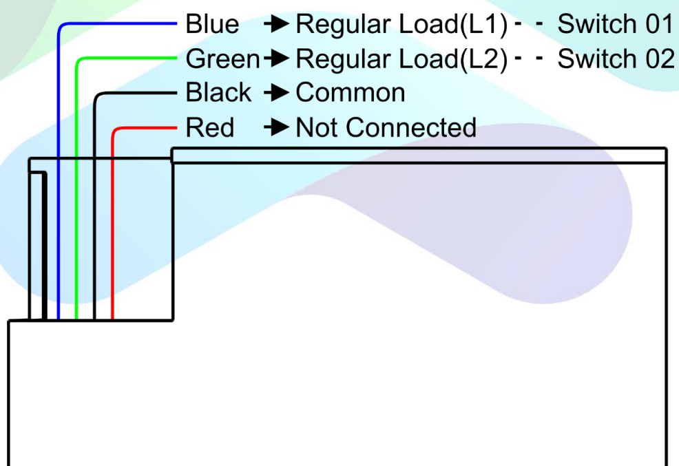
Smart Node Colour Wires to Switch Connection
