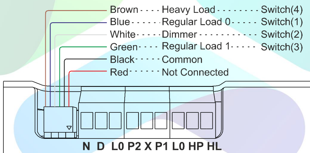
Smart Node Colour Wires to Switch Connection
