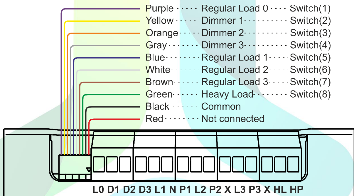
Smart Node Colour Wires to Switch Connection
