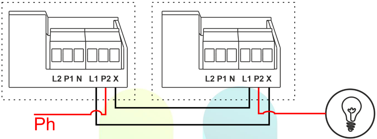
Switch Board 1
