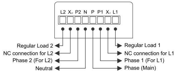
Wiring diagram
