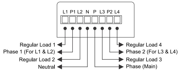
Wiring diagram
