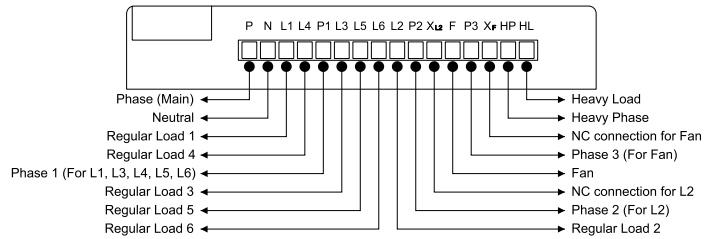
Wiring diagram
